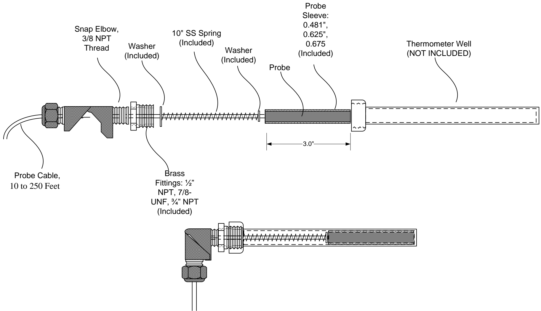
TTC-PROBE-01-zzz, Snap Elbow Probe Assembly Advanced Power Technologies, 215 State Route 10, Randolph, NJ, (973) 328-3300
